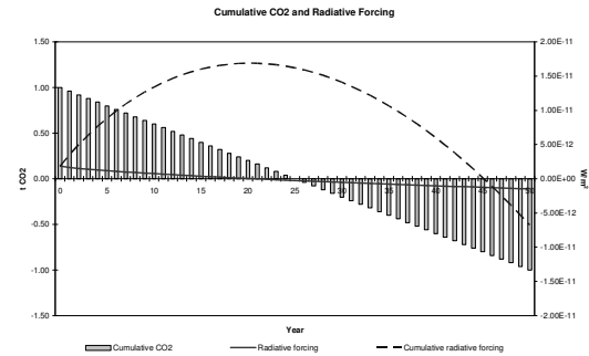
Figure 4: Comparison of cumulative emissions, radiative forcing and cumulative radiative forcing
