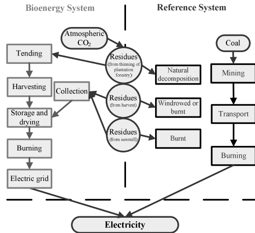
Figure 2: system diagram for integrated plantation forestry in North East NSW, Australia [4]
